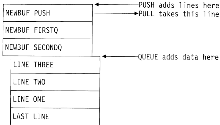
Figure 9-2. External data queue after ADDREXBUF
